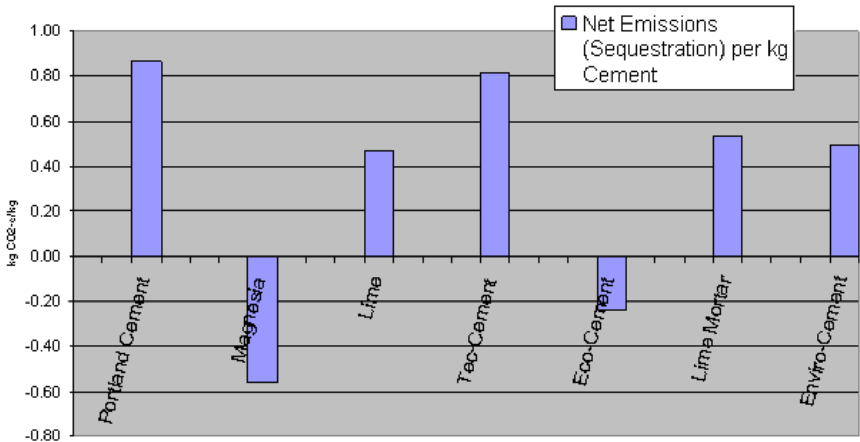
Net Emissions (Sequestration) per kg Cement
